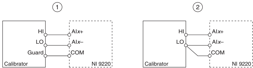
Figure 1. Accuracy Verification Connections
