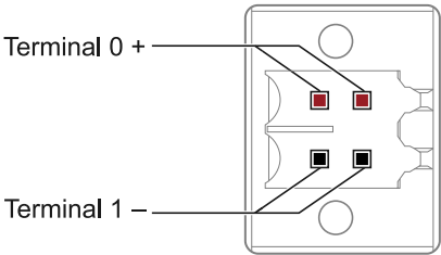
Figure 6. PXle-4112 Auxiliary Power Input Connector
