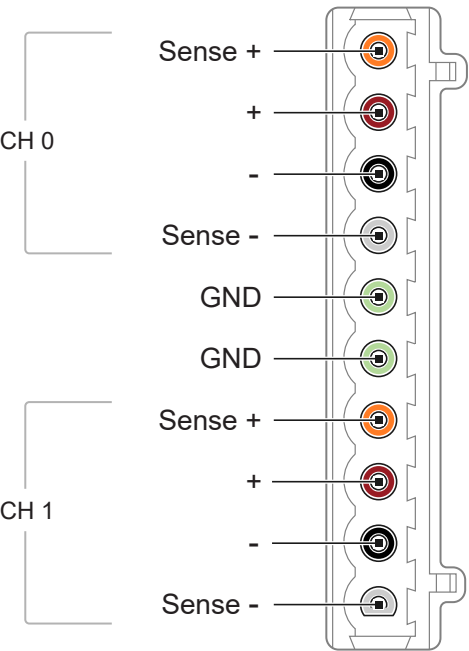
Figure 5. PXIe-4112 Output Connector Pinout
