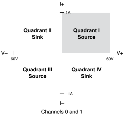
Figure 7. PXIe-4112 Quadrant Diagram
