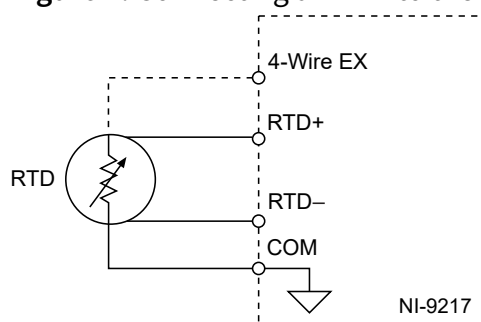
Figure 1. Connecting an RTD to the NI-9216
